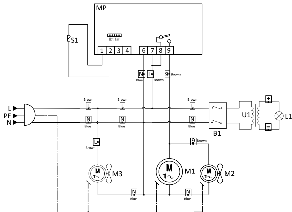
"Digital controller"
