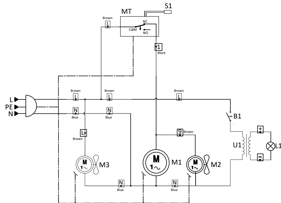
"Mechanical controller"
