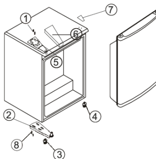
FIGURE 2 Door opening from right side
