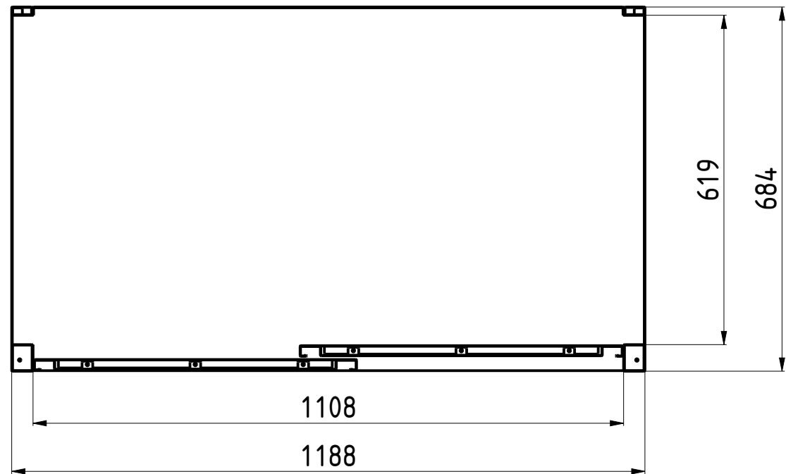
INTERNAL DIM D-D
