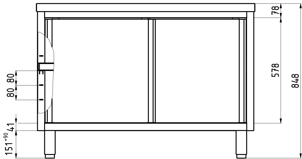
FRONT VIEW C-C 1:10
