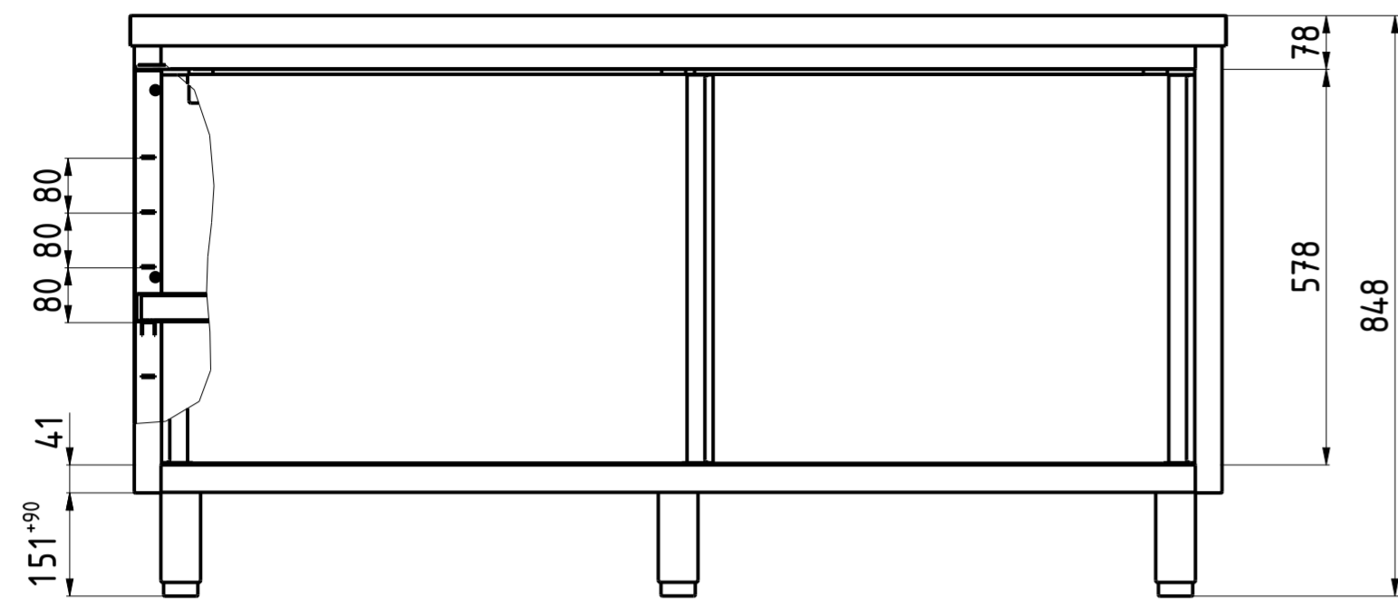
FRONT VIEW B-B 1:10
