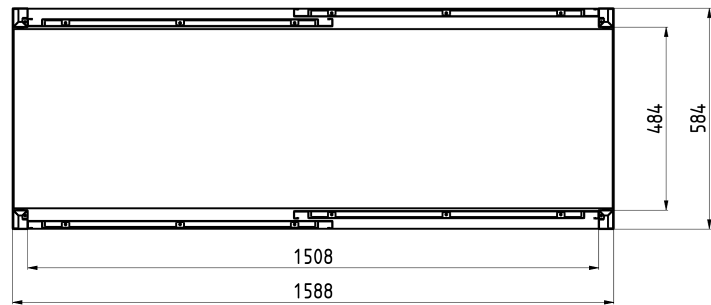
INTERNAL DIM C-C
