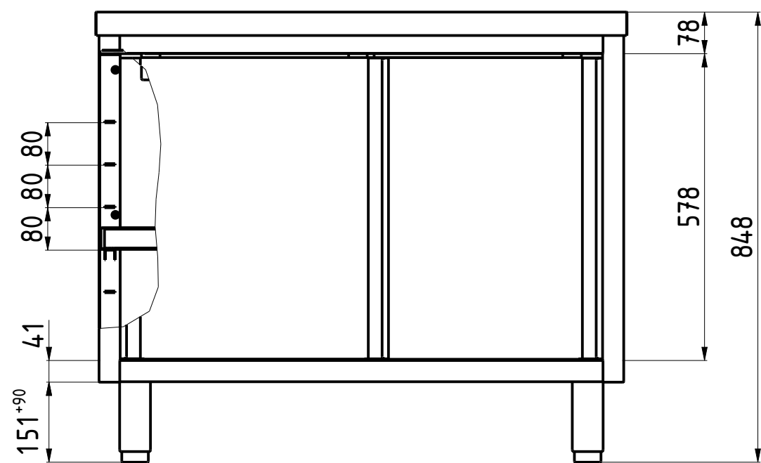
FRONT VIEW B-B 1:10
