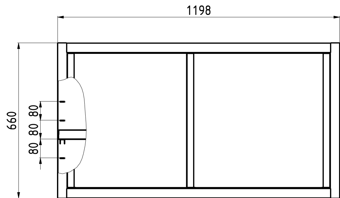
FRONT VIEW B-B 1:10
